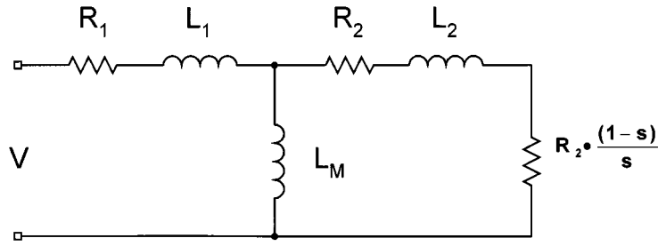
FIGURE 66.16 Equivalent circuit of ac induction motor.
