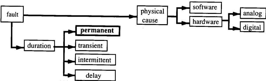
FIGURE 85.2 Fault characteristics.
