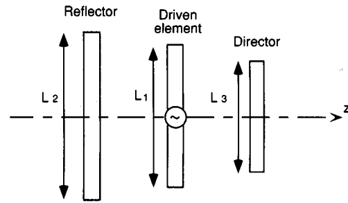
FIGURE 38.5 Three-element Yagi–Uda antenna. (Source: Shintaro Uda and Yasuto Mushiaki, Yagi–Uda Antenna , Sendai, Japan: Sasaki Printing and Publishing Company, 1954, p. 100. With permission.)
