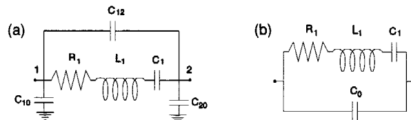
FIGURE 47.15 (a) Two-port resonator equivalent circuit and (b) one-port resonator equivalent circuit.
