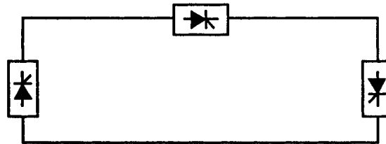
FIGURE 61.11 Series-connected MTDC system.
