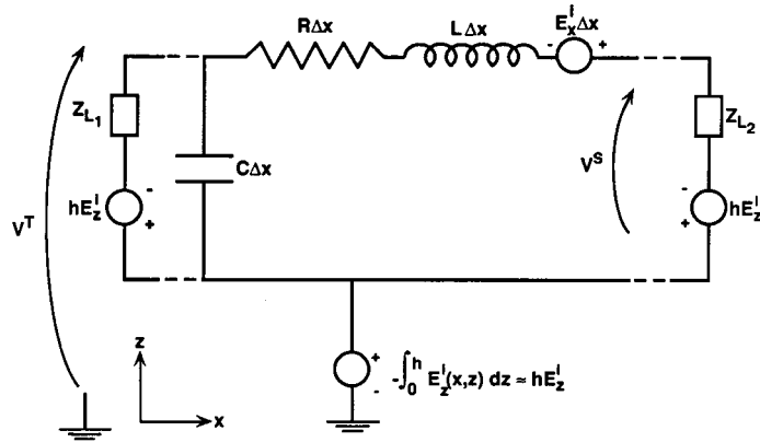
FIGURE 40.24 Equivalent circuit model obtained from Eqs. (40.17) through (40.19).
