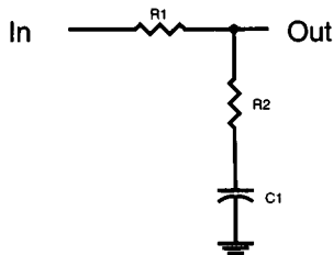
FIGURE 76.2 Passive loop filter.
