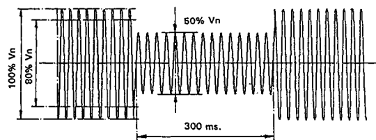
FIGURE 62.8 Voltage sag.
