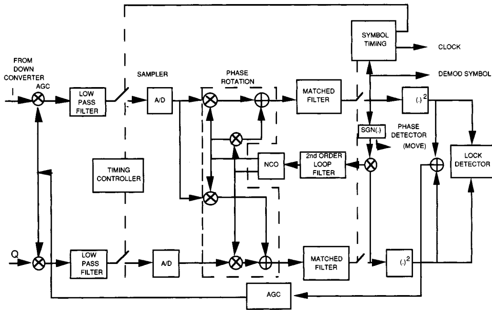
FIGURE 102.9 DSP demodulator functional diagram.
