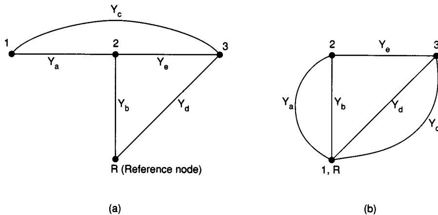
FIGURE 3.44 (a) Graph G , and (b) the modified graph G_i of G .
