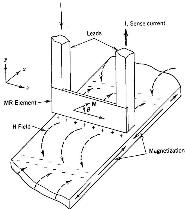
FIGURE 36.15 An unshielded magnetoresistive element. (Source: A.S. Hoagland and J.E. Monson, Digital Magnetic Recording , 2nd ed., New York: Wiley-Interscience, 1991, p. 131. With permission.)
