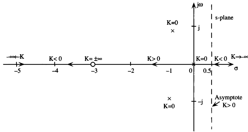
FIGURE 100.23 Some properties of the root loci of G(s)H(s) = K(s + 3)/[s(s^2 + 2s + 2)] .
