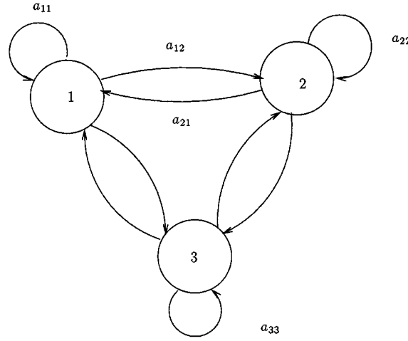
FIGURE 15.21 A first-order three-state hidden Markov model .
