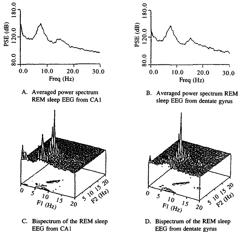
FIGURE 115.4 A and B represent the averaged power spectra of 80 4-s epochs of REM sleep (sampling rate = 128 Hz) obtained from hippocampal CA1 and the dentate gyrus, respectively. Note that both spectra exhibit clear power peaks at 7-Hz (theta) and 14-Hz (beta) frequencies. C and D represent the bispectrum of these same epochs from CA1 and the dentate gyrus, respectively. Computation of the bicoherence index at 7 Hz shows significant quadratic phase coupling at this frequency, indicating that the 14-Hz peak is not spontaneously generated, but results from quadratic phase coupling.
