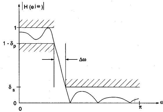
FIGURE 14.11 Frequency characteristics of an IIR digital low-pass filter showing definitions of passband ripple \delta_p , stopband attenuation \delta_s , and transition bandwidth \Delta\omega .
