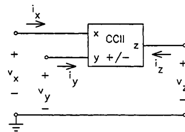
FIGURE 29.26 A CCII current conveyor.
