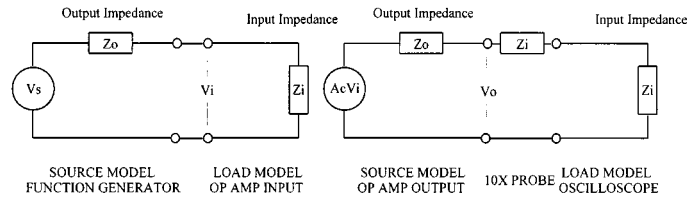
FIGURE 108.5 Model of representative instrumentation system. Each variable would be substituted as required. For example, V_s = 1.0\sin 2\pi 1000t for a 0.707 Vrms, 1 kHz sine wave; Z_o = 50\ \Omega for the FG501A; Z_i = 1\ \text{k}\Omega for an op amp configured as an inverting amplifier with R_i = 1\ \text{k}\Omega ; and gain of 10; AcVi = -10.0\sin 2\pi 1000t ; Z_o = 1\ \Omega for low current output; Z_i = 9\ \text{M}\Omega || 1.4\ \text{pF} for a compensated 10X probe; and with Z_i = 1\ \text{M}\Omega || 13\ \text{pF} for the input model of the HP54601A oscilloscope.
