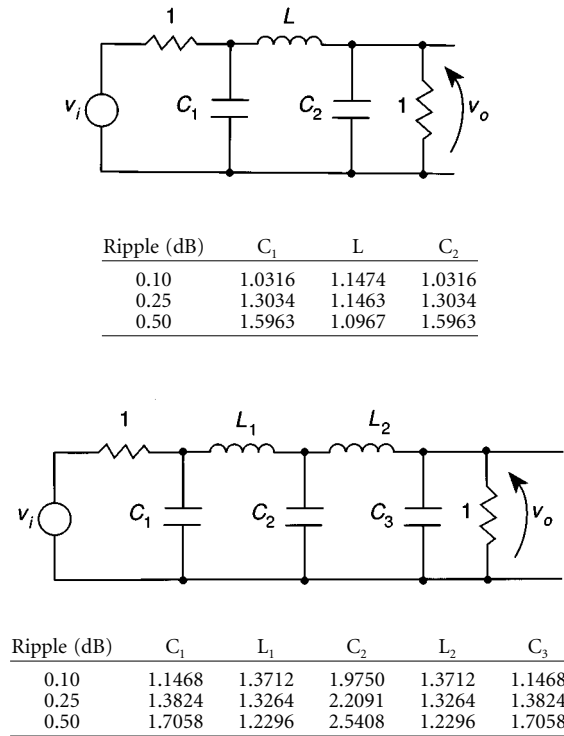
FIGURE 4.7 Doubly terminated Chebyshev filter element values (in \Omega , H, F).
