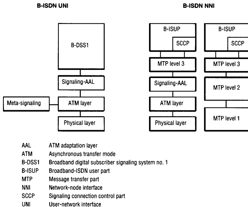
FIGURE 72.4 Protocol stacks for B-ISDN signaling.
