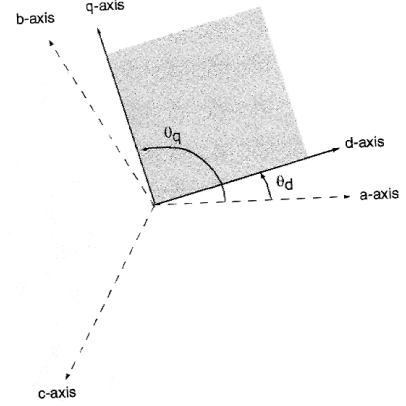
FIGURE 66.33 qd0 transformation.
