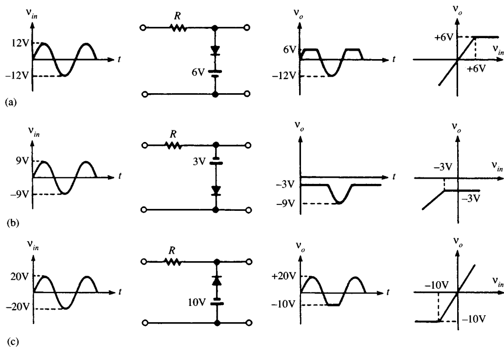
FIGURE 5.12 Examples of parallel clipping circuits. (Source: T.F. Bogart, Jr., Electronic Devices and Circuits , 3rd ed., Columbus, Ohio: Macmillan/Merrill, 1993, p. 692. With permission.)
